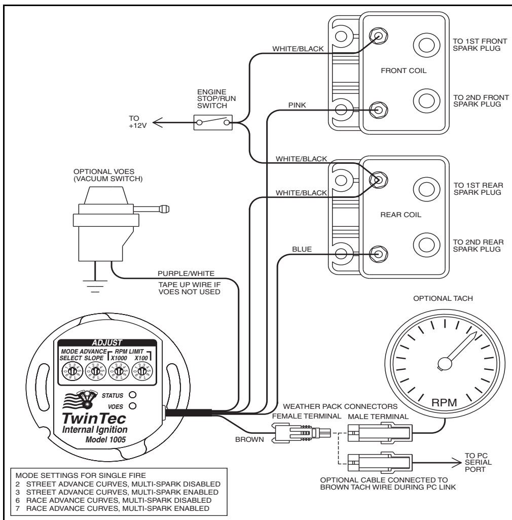
Figure 1 – Model 1005/1005S Dual Spark Plug Wiring Diagram
