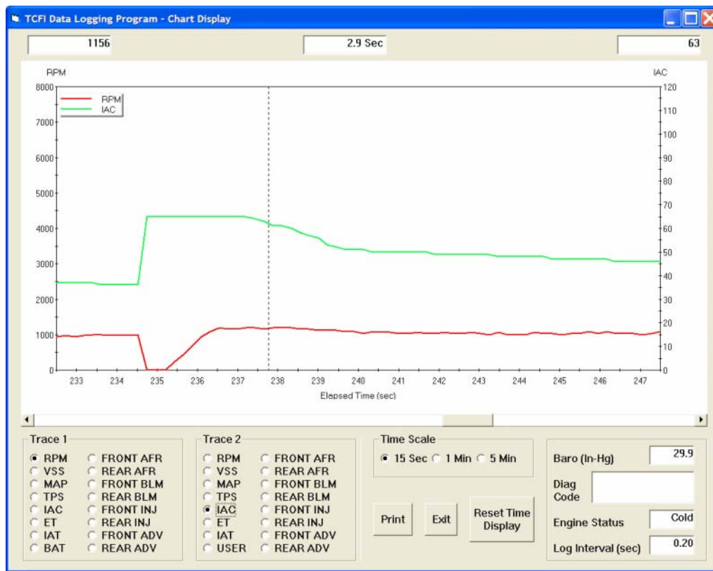
Figure 4 – Hot Start Test with Correct IAC Start Adder
