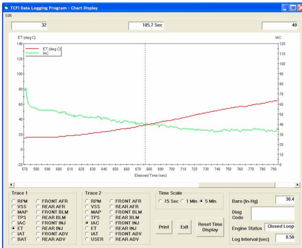
Figure 3 – Cold Start Test Showing ET and IAC Data
