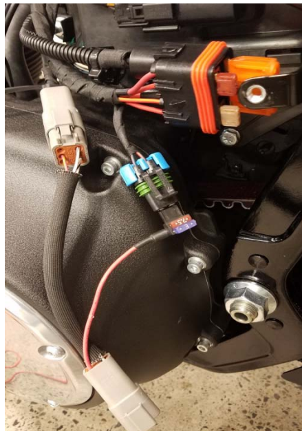
Figure 19C – SYSTEM 7.5A Fuse tap connection for switched uninterrupted power on 2018
