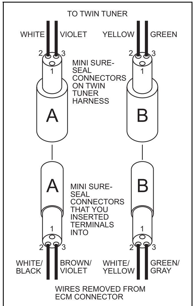
Figure 4 – Twin Tuner Wiring
