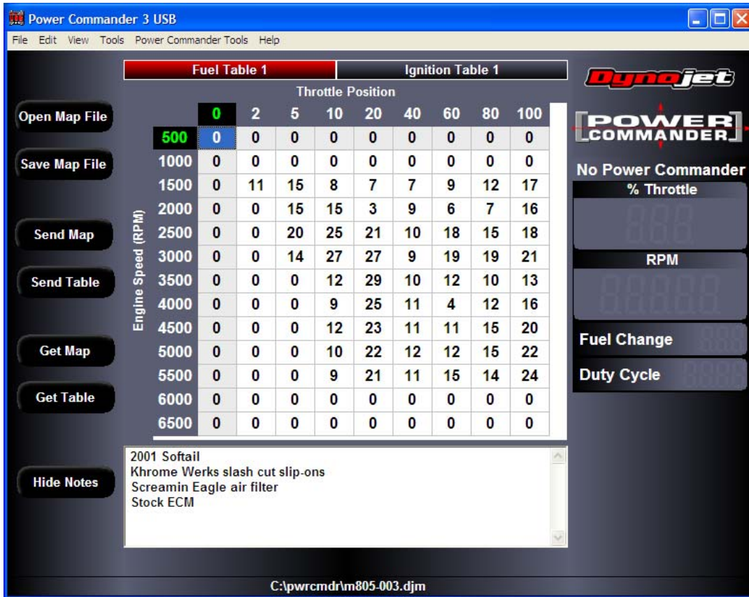
Figure 13 – Typical Dynojet Power Commander Fuel Table
