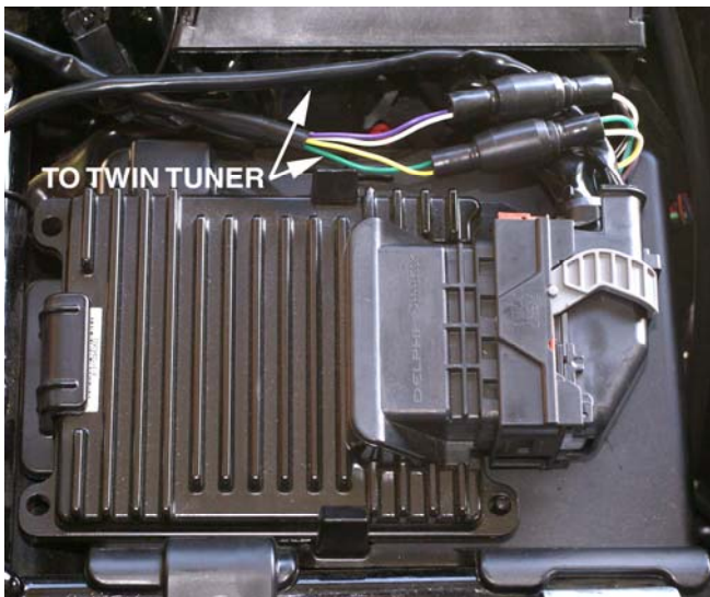
Figure 7 – Completed Wiring at ECM
